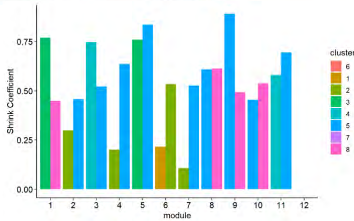
Figure 9. The top two learning tactic clusters that have the largest shrink factor for each of the 11 modules in the learning module sequence. The bar heights correspond to the magnitudes of the shrink factor, and the colour corresponds to the learning tactic cluster.
