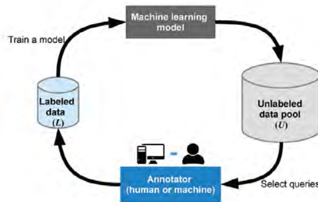
Figure 2. The iterative active learning process integrated with semi-supervised learning.
