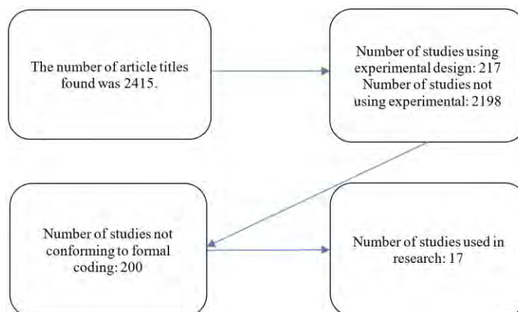
Figure 1. PRISMA
