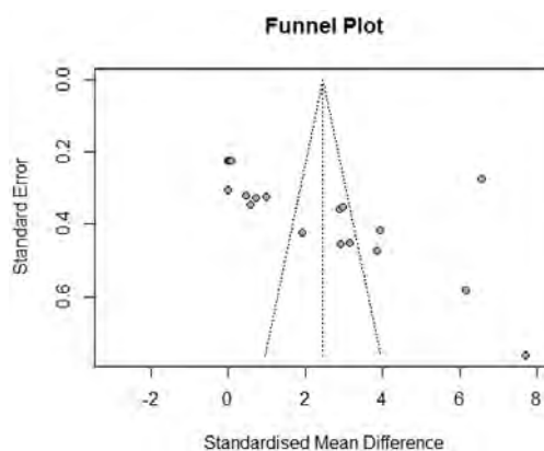
Figure 2. Funnel plot
