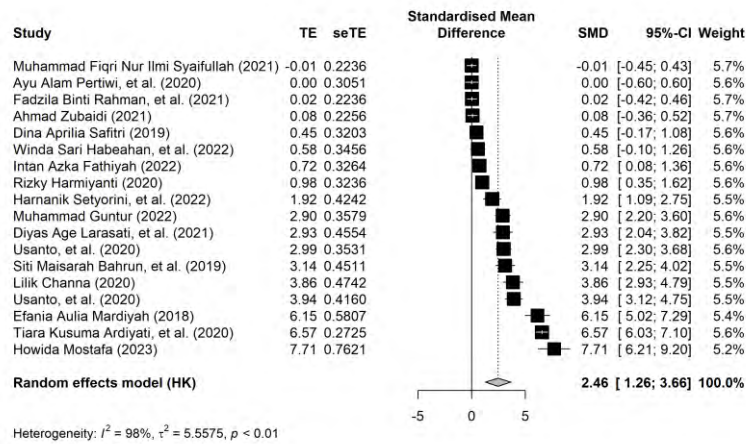
Figure 5. Forest plot
