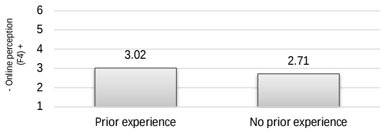
Figure 2 Likert-scale averages for prior experience with online classes and F4 (Online is fine)
