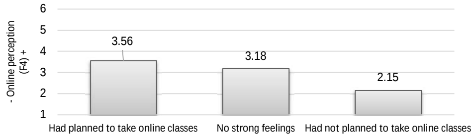
Figure 3 Likert-scale averages for desire for online classes and F4 (Online is fine)
