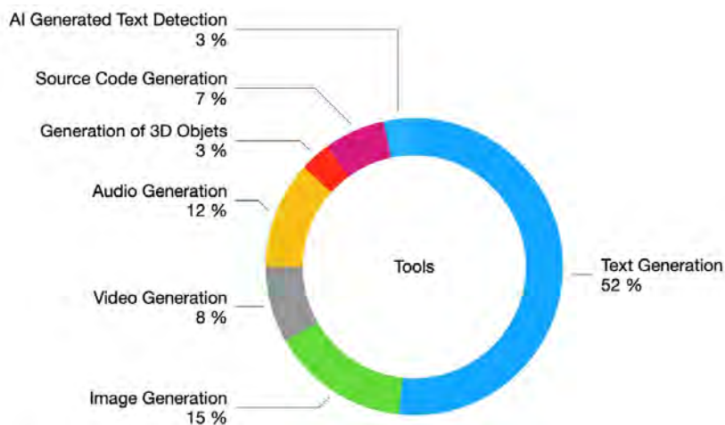
Figure 2. AI tools
