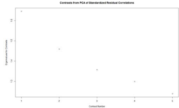
Figure 3. Contrasts from PCA of standardized residual correlations
