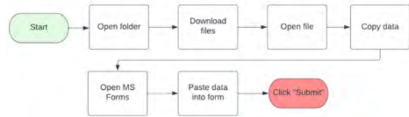
Figure 3. Flowchart Example
