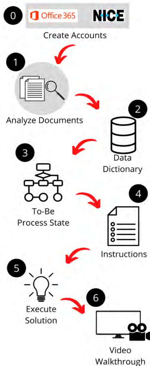
Figure 1. Workflow
