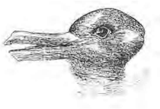
Figure 1: Duckrabbit ambiguity
