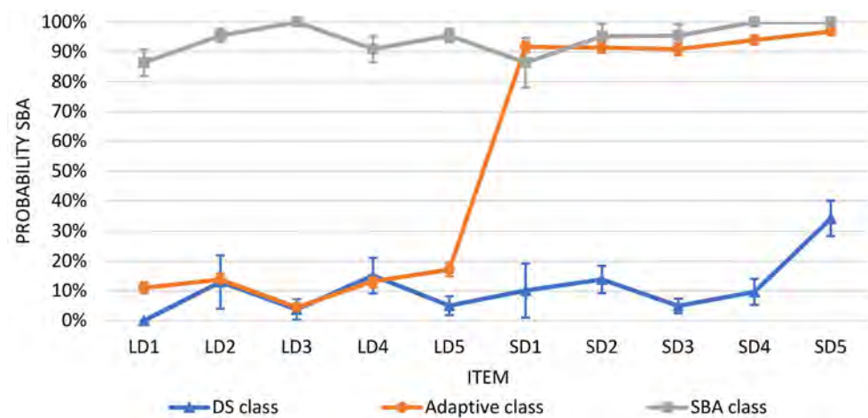
Probability to Use Subtraction by Addition (and SE) on the Ten Items in the Choice Condition for the Three Classes
