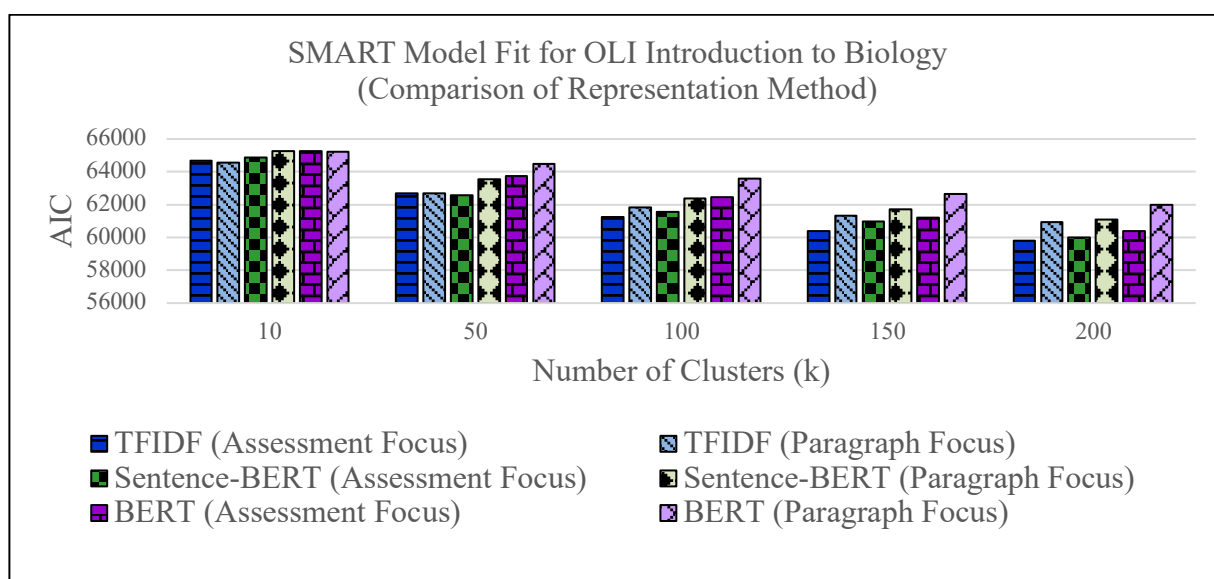
Figure 6. Comparison of the results of the model fit for SMART with varying representation methods on the OLI Introduction to Biology course.
