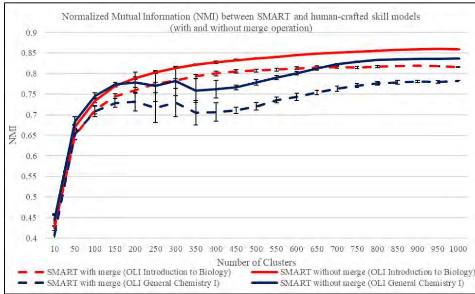
Figure 5. Normalized Mutual Information (NMI) between SMART skill models (with and without merging clusters) and the human-generated skill model for OLI Introduction to Biology and OLI General Chemistry I.
