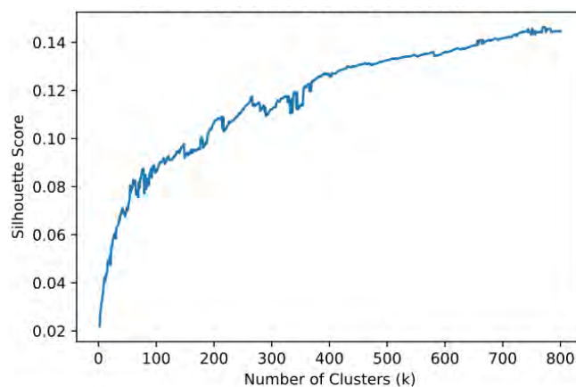
Figure 9. Measurement of the silhouette score for clustering assessment items as the number of clusters increases (OLI General Chemistry 1 course).
