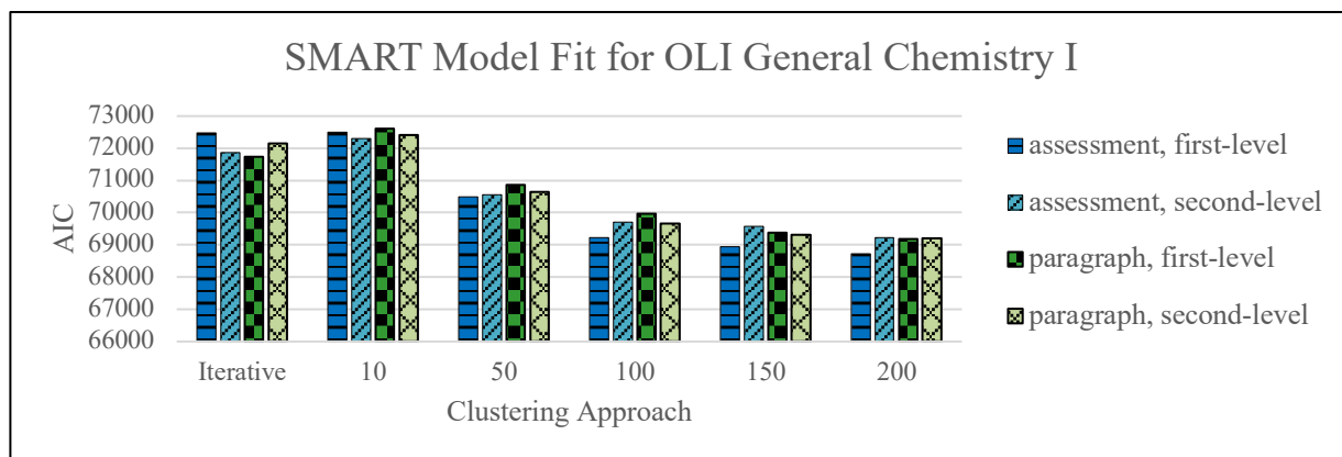
Figure 4. Results of the model fit for SMART on OLI General Chemistry I across the range of hyperparameter values.
