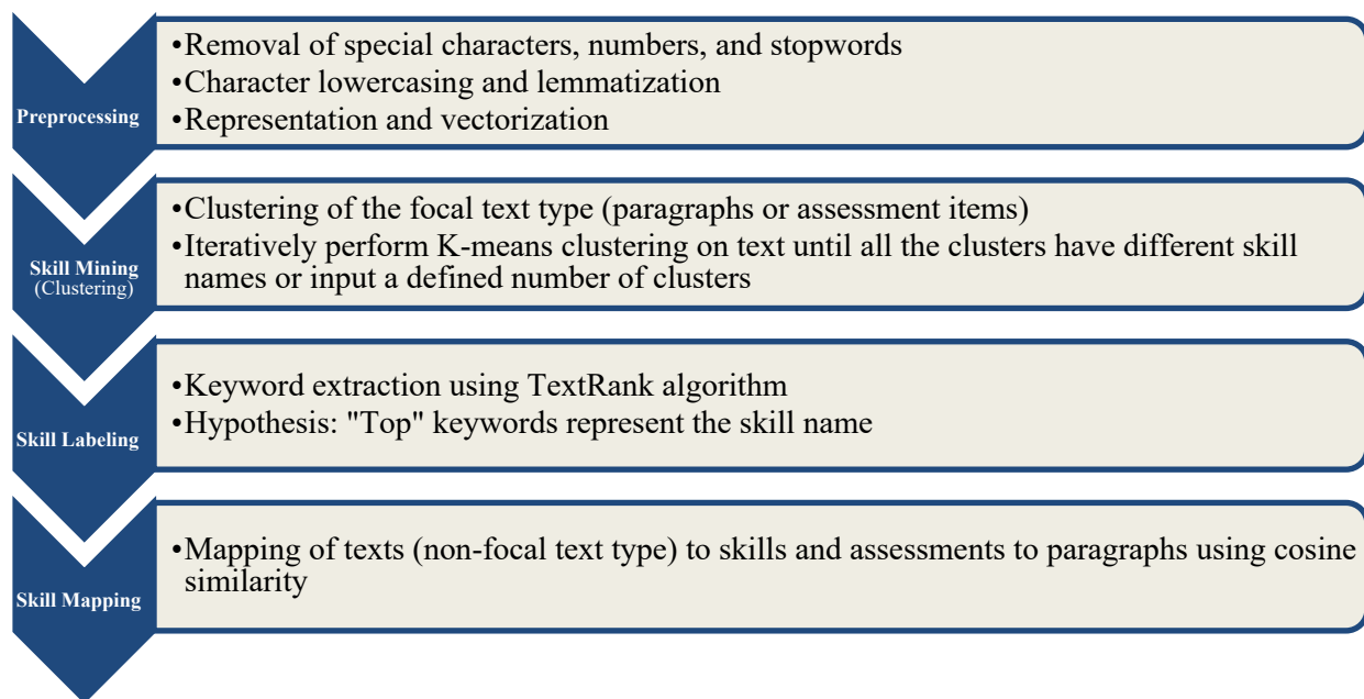
Figure 2. Multi-step process depicting the SMART method.
