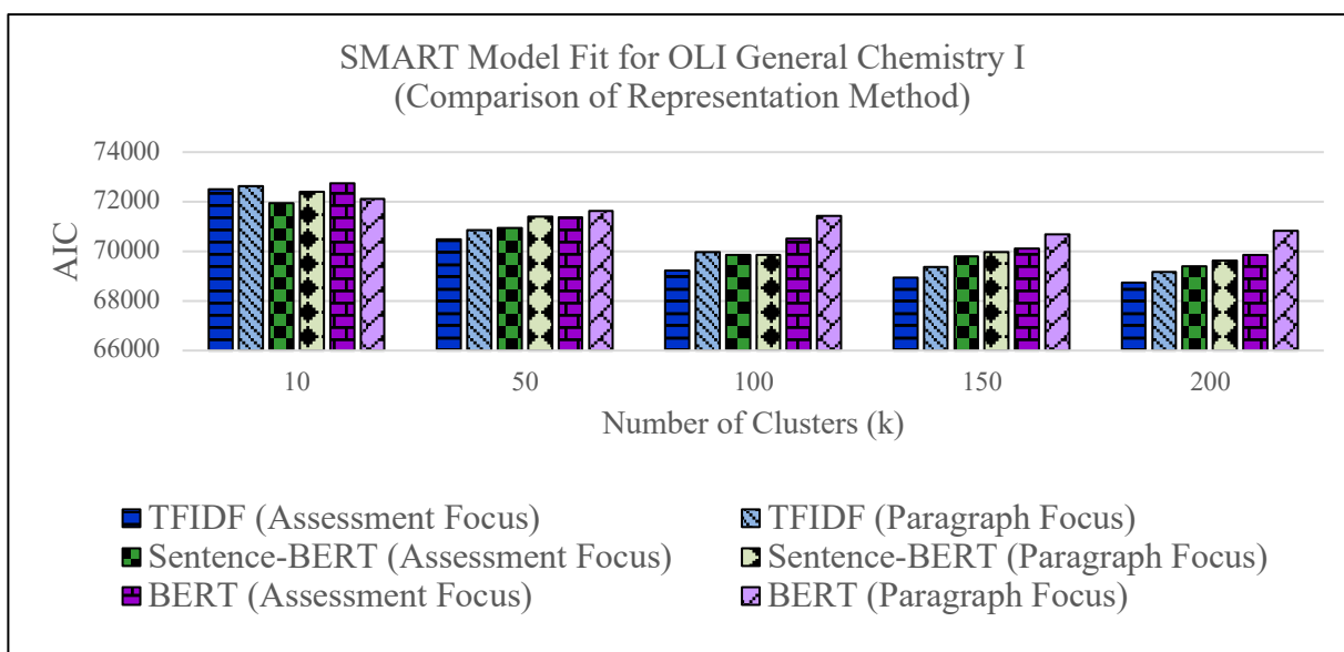
Figure 7. Comparison of the results of the model fit for SMART with varying representation methods on the OLI General Chemistry I course.
