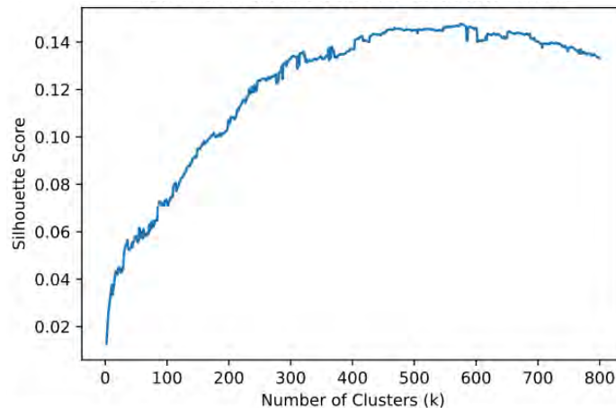
Figure 8. Measurement of the silhouette score for clustering assessment items as the number of clusters increases (OLI Introduction to Biology course).
