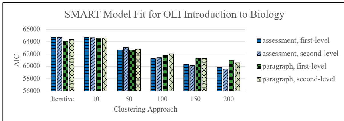
Figure 3. Results of the model fit for SMART on OLI Introduction to Biology across the range of hyperparameter values.
