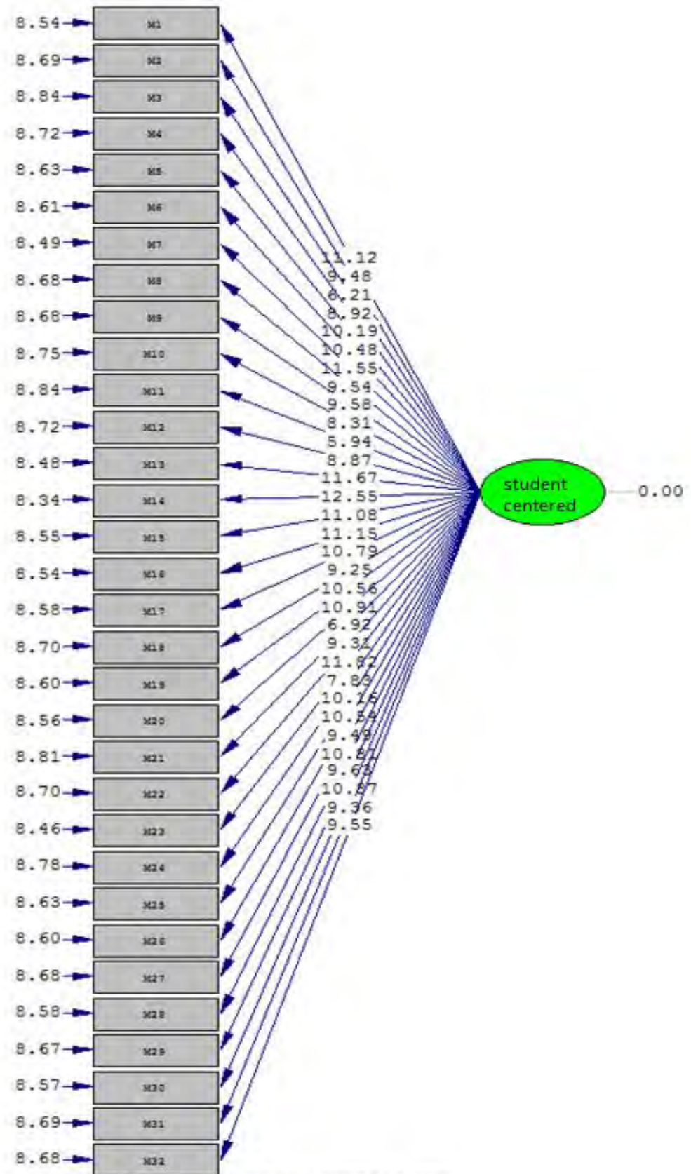
Figure 3. Confirmatory Factor Analysis Model (t-values)
