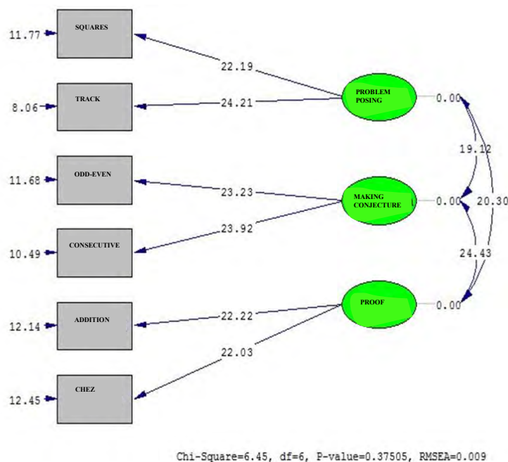
Figure 2. Path Diagram of the MCT-CFA Results
