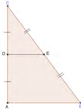
Fig 3. Illustration of the triangle ABC
