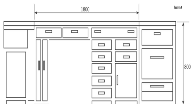
Figure 8. The teacher table plan (Chung, 2004)
