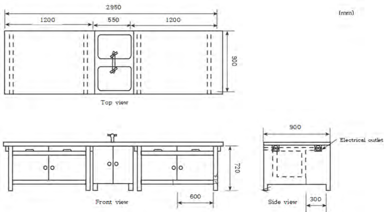
Figure 5. The table plan (Chung, 2004)
