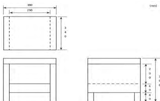
Figure 7. The chair plan (Chung, 2004)
