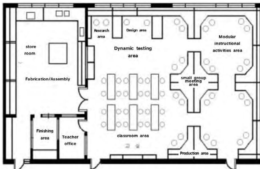
Figure 2. Technology education facility
