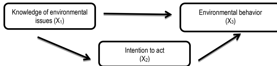
Figure 1. Path analysis
