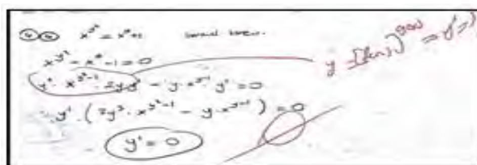
Figure 9. Thinking of every function as polynomial function when evaluating a derivative
