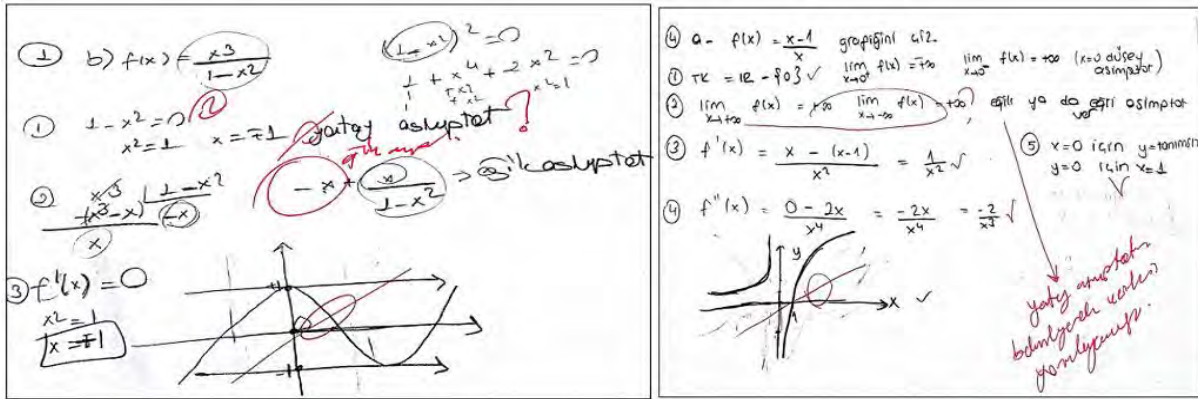
Figure 6. Failure to determine the asymptotes
