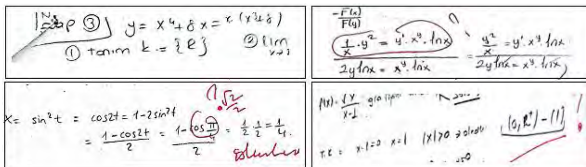
Figure 8. Failure to use mathematical statements (notations) properly
