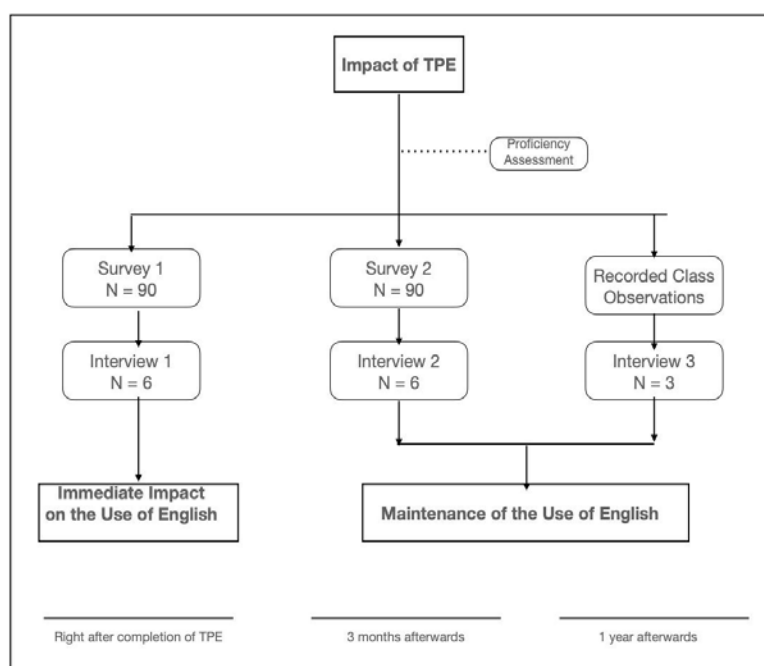
Figure 1. Research Design
