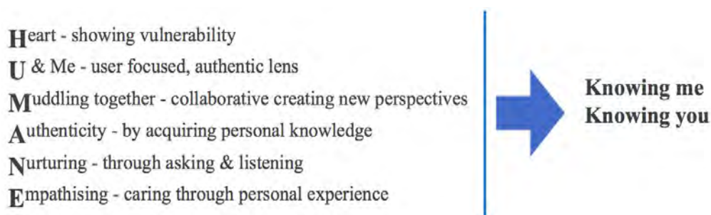
Figure 1: HUMANE framework
