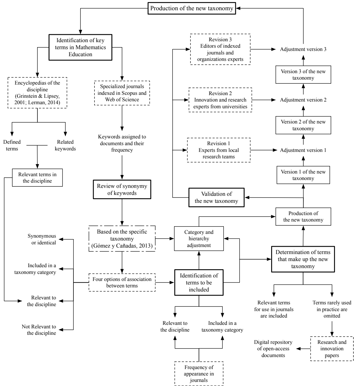
Figure 3. Production Process of the New Taxonomy
