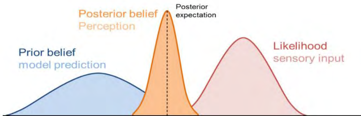
Figure 1. Calculation of Bayesian posterior probability. source: Adams et al. (2013)
