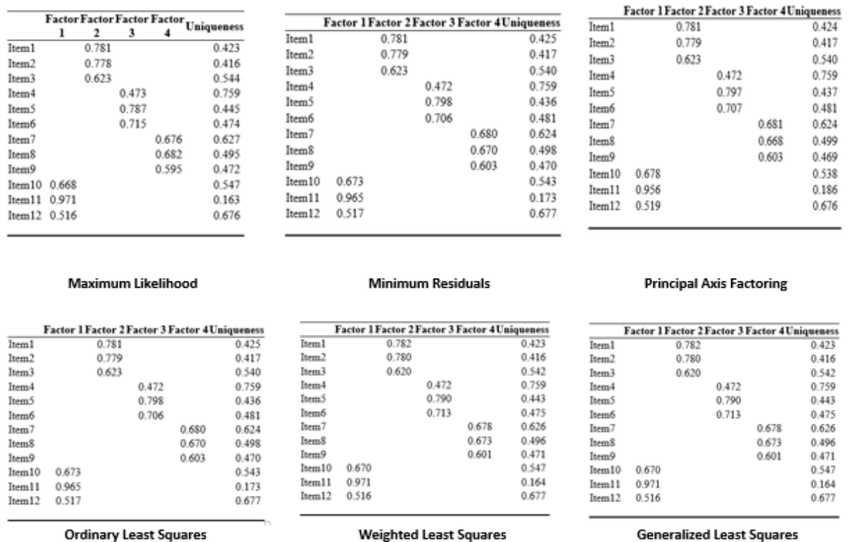
Figure 3. Factor loading tables for different factor extraction methods
