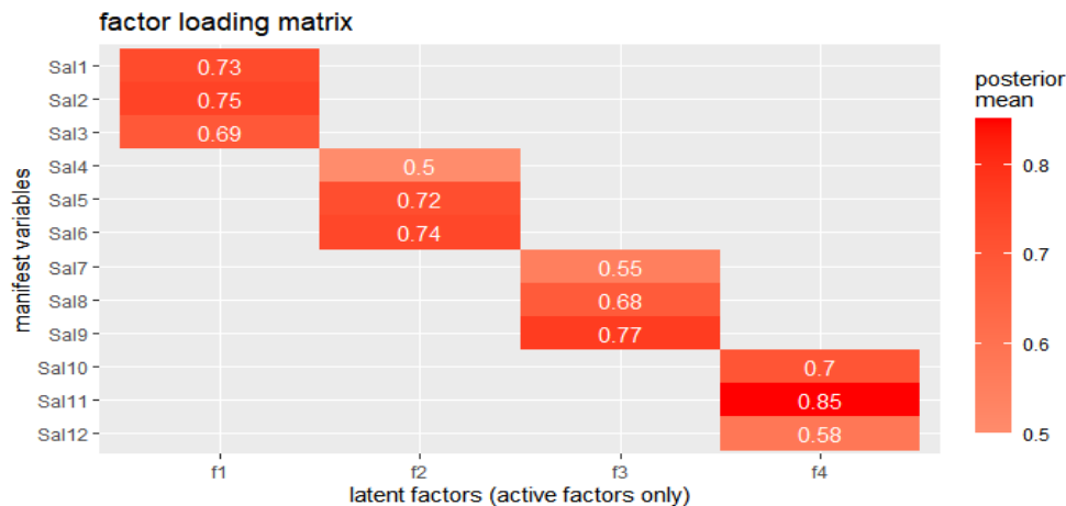
Figure 4. Factor loading matrix
