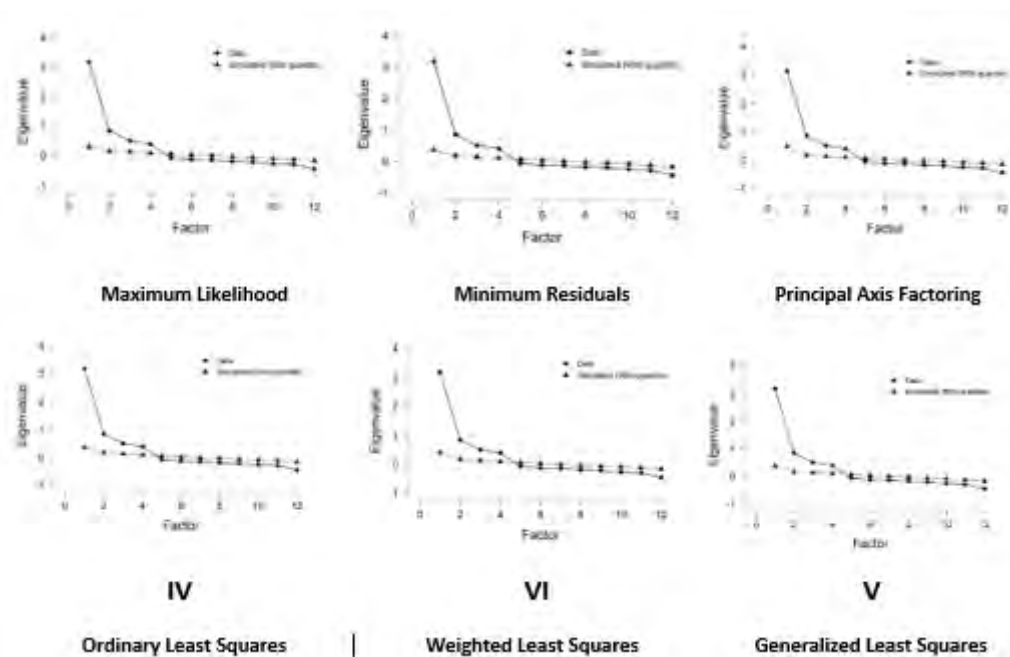
Figure 2. Scree plots of factor extraction methods
