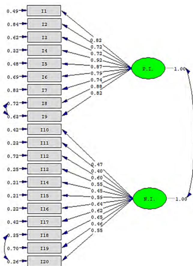
Figure 2. Path diagram of two-dimensional model post-modification.
