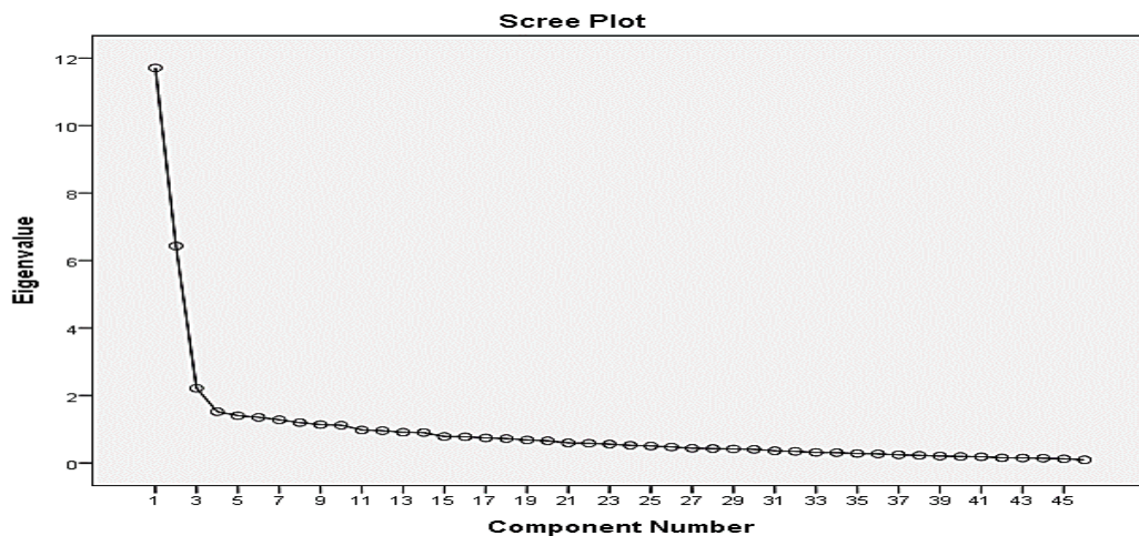
Figure 1. Scree plot for factor solution of items in the OTDAS.
