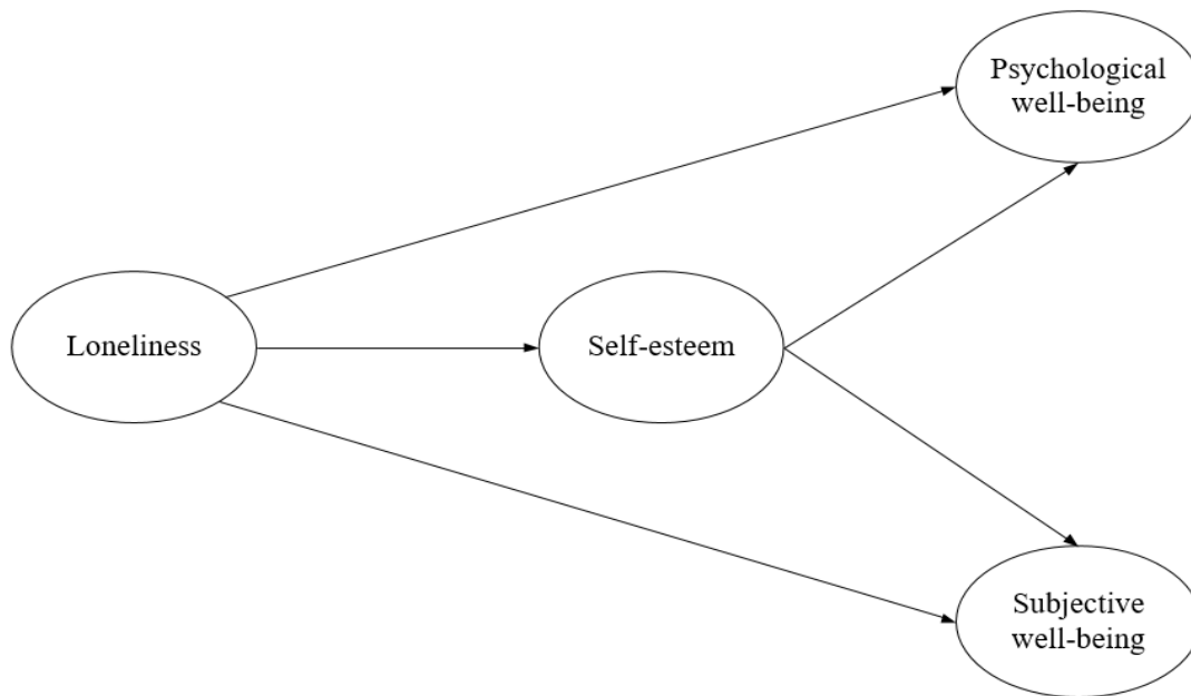
Figure 1. The proposed model of relationships between variables
