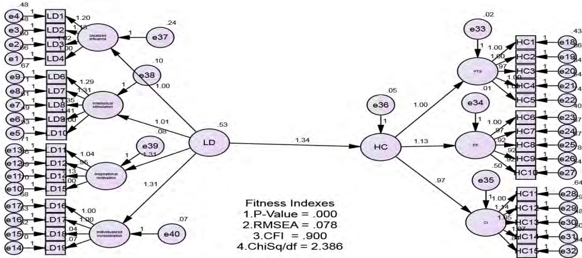
Figure 3 Regression Weight
