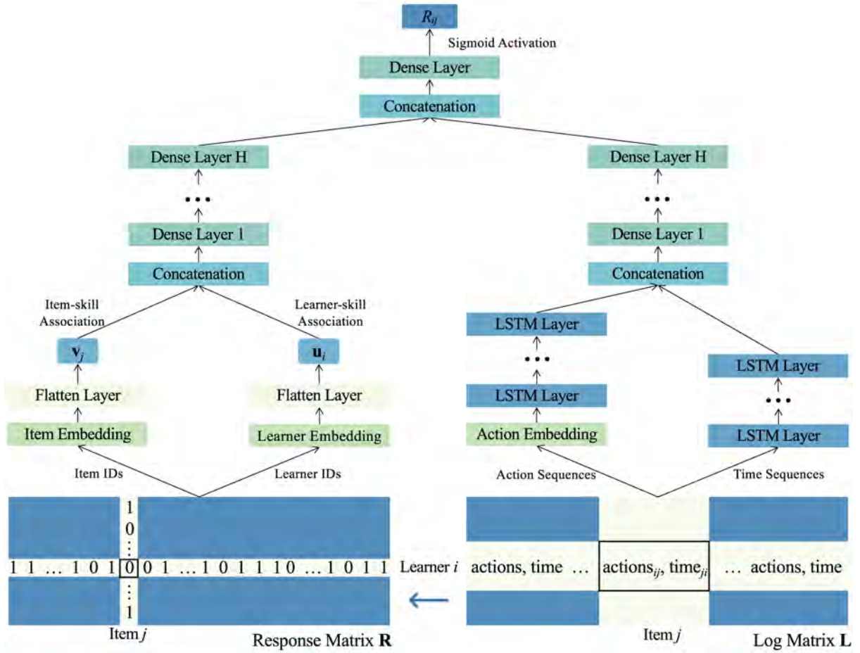
Figure 1: General framework of deep CF with process data.
