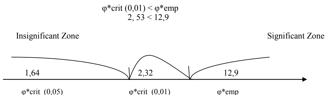
Figure 1. Graphical F-test presentation with Significant and Insignificant zones
