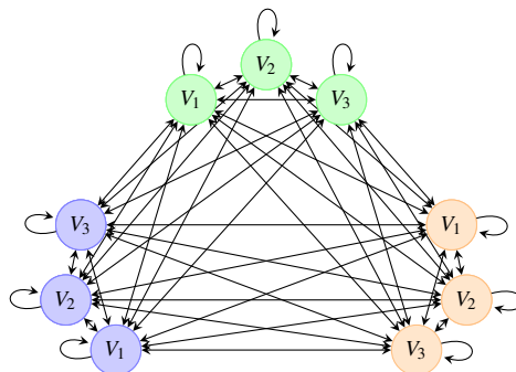
Figure 1. Representation of collaborative process data as a fully connected dynamical network. Nodes represent group members’ actions, the node colour represents the group member who performed the action, and the node name represents the type of action. The edges represent temporal statistical dependence among the nodes.
