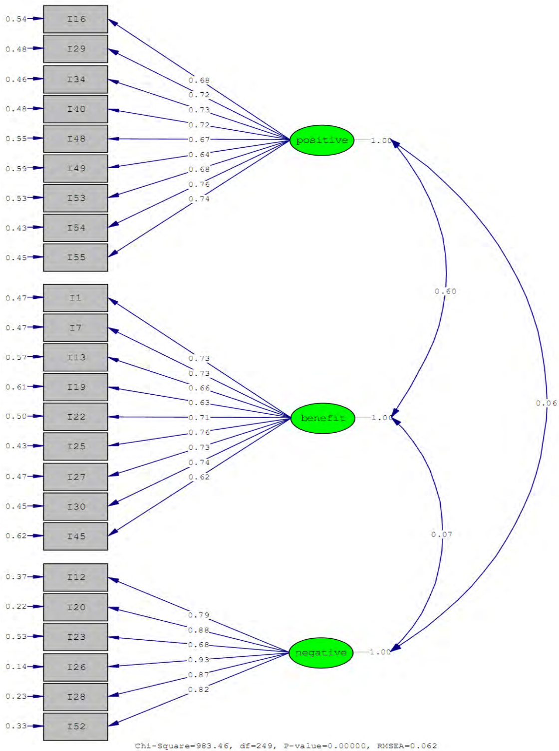
Figure 2 The model obtained as a result of confirmatory factor analysis
