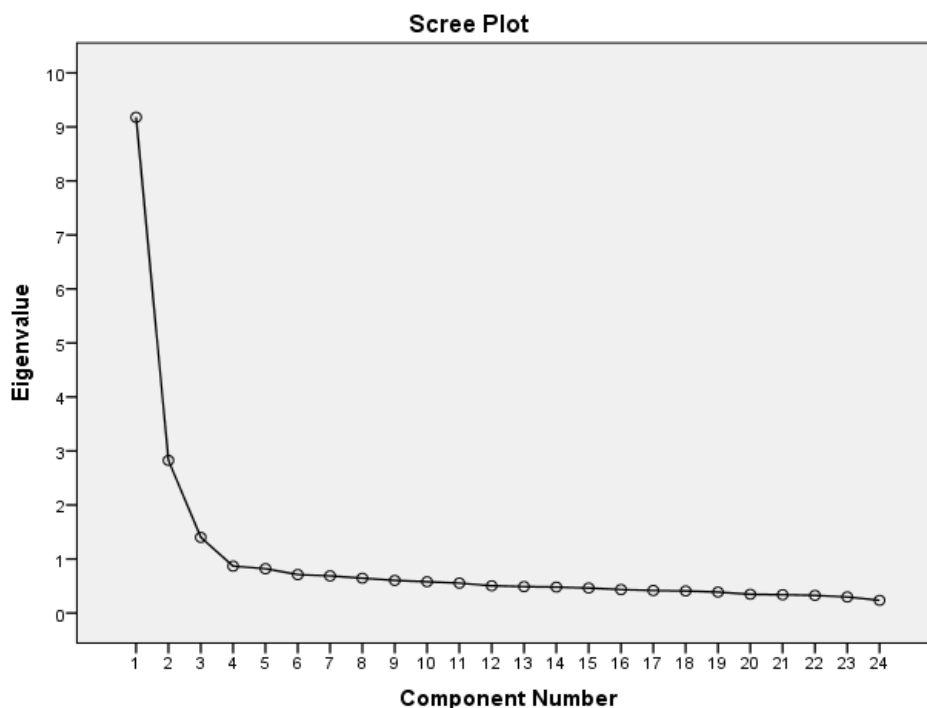
Figure 1 Scree-plot graphic of the scale
