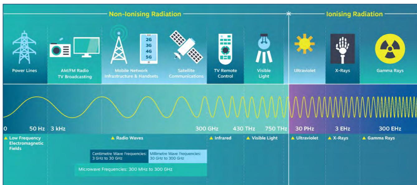
Figure 1 Electromagnetic spectrum
