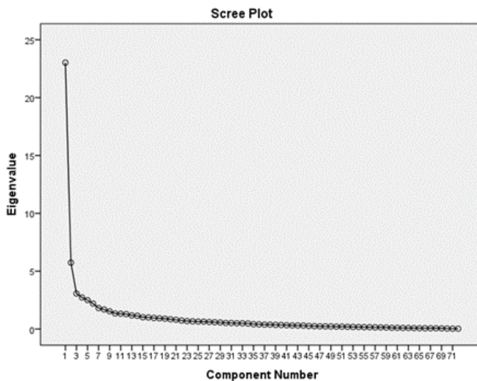
Figure 1. Scree Plot Graph of the Scale
