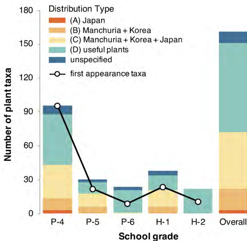
Figure 3. Summary of cited plant taxa in science textbooks for Japanese students in Manchuria. The stacked bar graphs indicate the number of taxa, shown by school grade (see Appendix 2). The plant species were categorized into four types based on geographical distribution and usage. The line graph represents the number of taxa introduced in each grade
