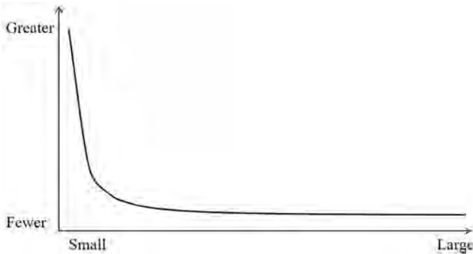
Figure 2 The asymptotic, long-tail curve of a power-law distribution
