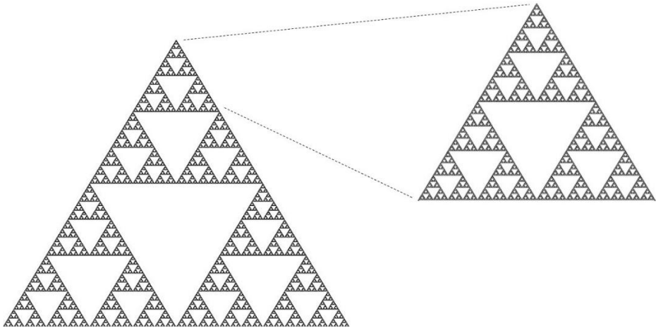
Figure 1 The Sierpiński triangle
