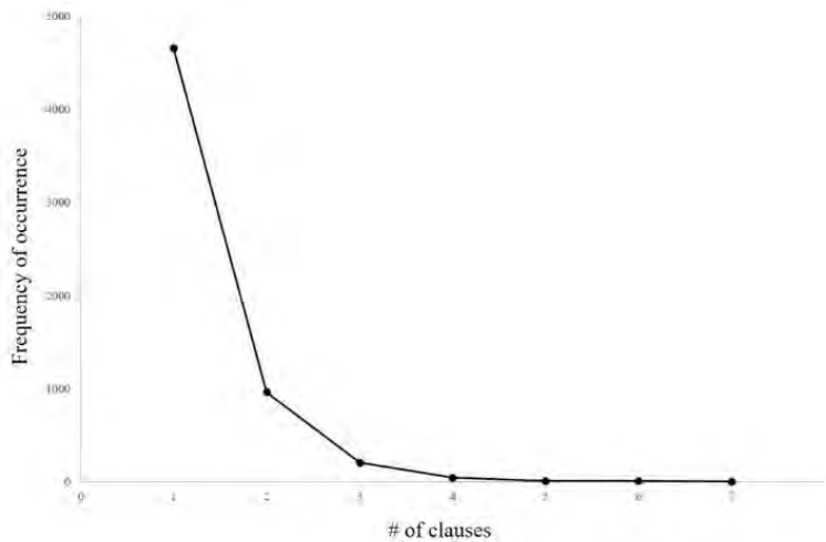
Figure 3 The frequency/density distribution of clausal density over 30 weeks
