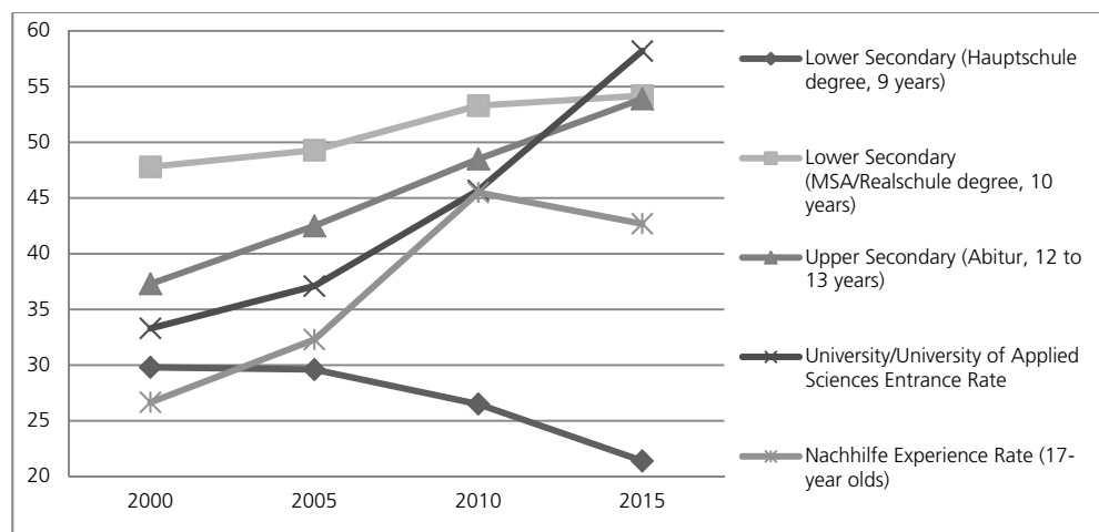
Figure 1. Percentage of Secondary Education Graduates, Entrants to Higher Education and Participation in Paid Nachhilfe in Germany (2000-2015)
