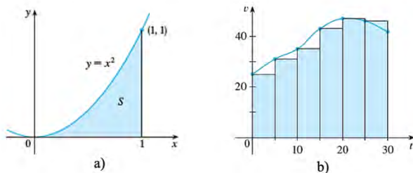
Figure 2. a) Area under a curve; b) Distance traveled
