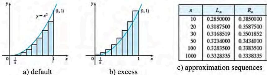
Figure 3. Approximating rectangles
