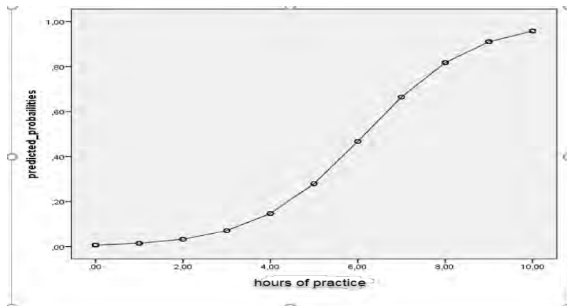
Figure 3 - predicted probabilities
