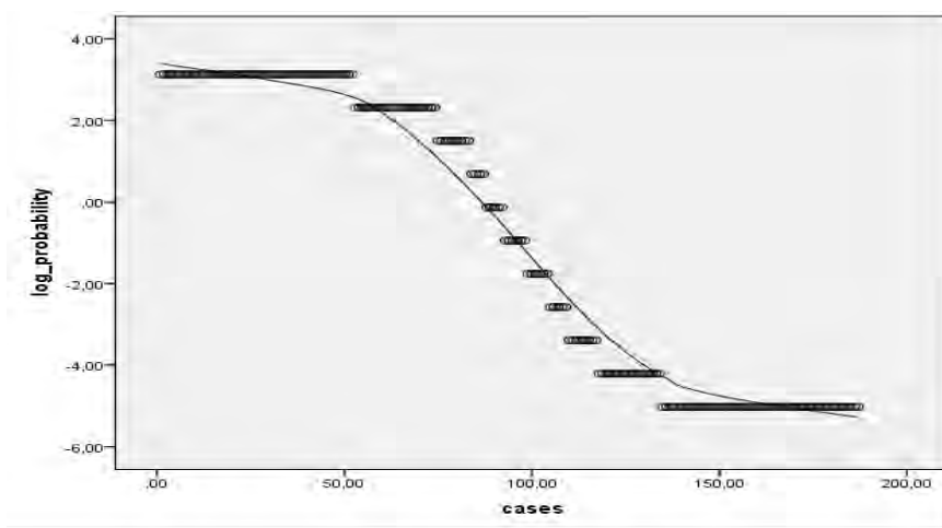
Figure 2 - log probabilities
