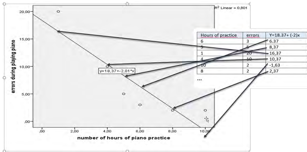
Figure 1- linear regression (OLS)
