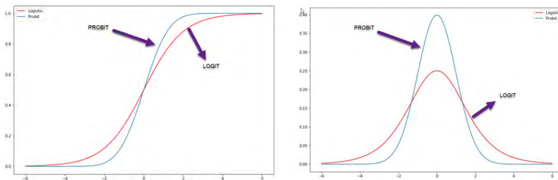
Figure 6 - logit and probit distribution
