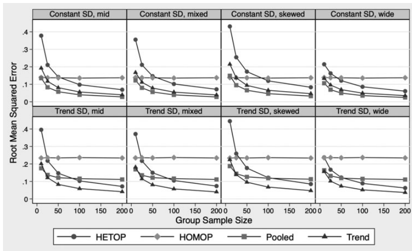
FIGURE 2. Root mean squared error of estimated standard deviations (SDs) by SD structure, cut score type, and sample size for each model. Constant SD and trend SD refer to different patterns of true group standard deviations described in text. The mid, skewed, wide, and mixed headings refer to different cut score locations; mid = symmetric cut scores at approximately the 20th/50th/80th percentiles; skewed = asymmetric cut scores at approximately the 5th/50th/95th percentiles; mixed = mix of mid/skewed/wide cut score locations across grades; HETOP = heteroskedastic ordered probit model; HOMOP = homoskedastic ordered probit model; pooled = fully pooled HETOP model; trend = linear trend pooled HETOP model.
