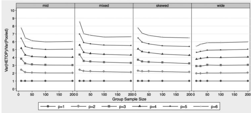
FIGURE 3. Efficiency ratios between HETOP and pooled HETOP models by cut score type, sample size, and number of pooled grades in the constant SD condition. The “ p ” refers to the number of grades used to estimate the fully pooled HETOP model. The mid, skewed, wide, and mixed headings refer to different cut score locations; mid = symmetric cut scores at approximately the 20th/50th/80th percentiles; skewed = asymmetric cut scores at approximately the 5th/30th/55th percentiles; wide = symmetric cut scores at approximately the 5th/50th/95th percentiles; mixed = mix of mid/skewed/wide cut score locations across grades.
