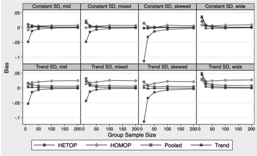
FIGURE 1. Bias in estimated standard deviations (SDs) by SD structure, cut score type, and sample size for each model. Constant SD and trend SD refer to different patterns of true group standard deviations described in text. The mid, skewed, wide, and mixed headings refer to different cut score locations; mid = symmetric cut scores at approximately the 20th/50th/80th percentiles; skewed = asymmetric cut scores at approximately the 5th/30th/55th percentiles; wide = symmetric cut scores at approximately the 5th/50th/95th percentiles; mixed = mix of mid/skewed/wide cut score locations across grades; HETOP = heteroskedastic ordered probit model; HOMOP = homoskedastic ordered probit model; pooled = fully pooled HETOP model; trend = linear trend pooled HETOP model.
