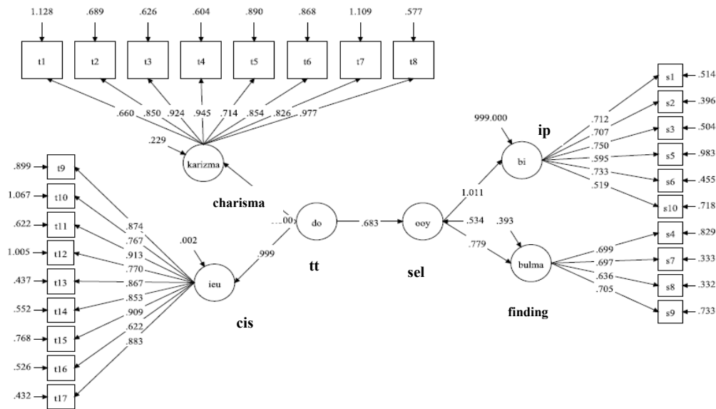
Figure 2. Path analysis
