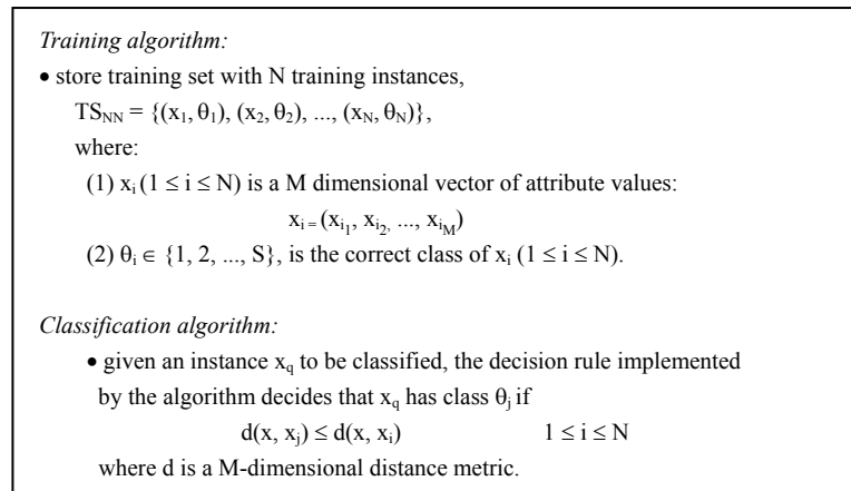
Figure 1. High level pseudocode of the Nearest Neighbor (NN) (Cover & Hart, 1967)
