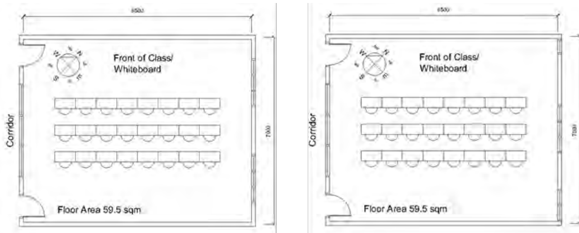
Fig. 2 Classroom One (left) and Two (right) Floor Plan
