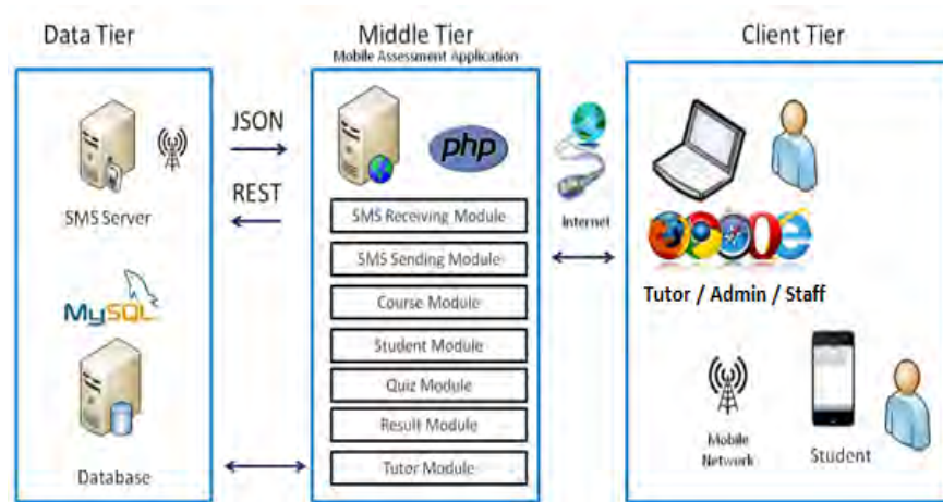
Figure 3: Three-Tier Architectural Model
