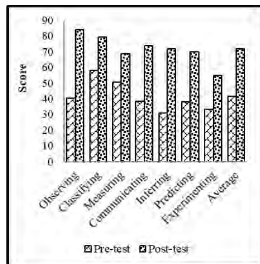
Figure 2. Students' science process skills: SDN Pasar Lama 3
