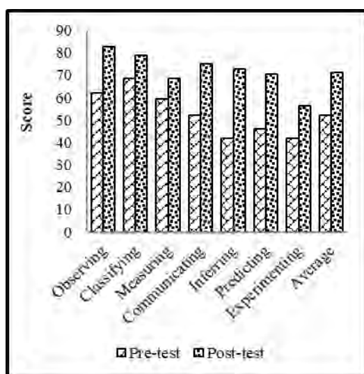
Figure 1. Students' science process skills: SDN Pasar Lama 1
