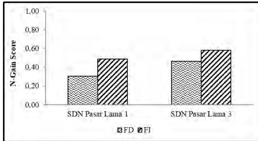
Figure 3. Improvement of the students' science process skills
