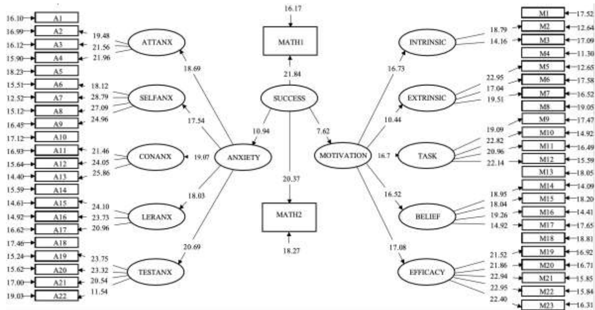
(Chi square=3667.52, sd=1030, p\text{-value}=0.000, RMSEA=0.057 ) Figure 2. t -values
