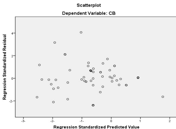
Figure 3. Scatterplot
