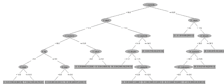
Figure 2. Decision Tree Obtained with the help of the REPTree Algorithm
