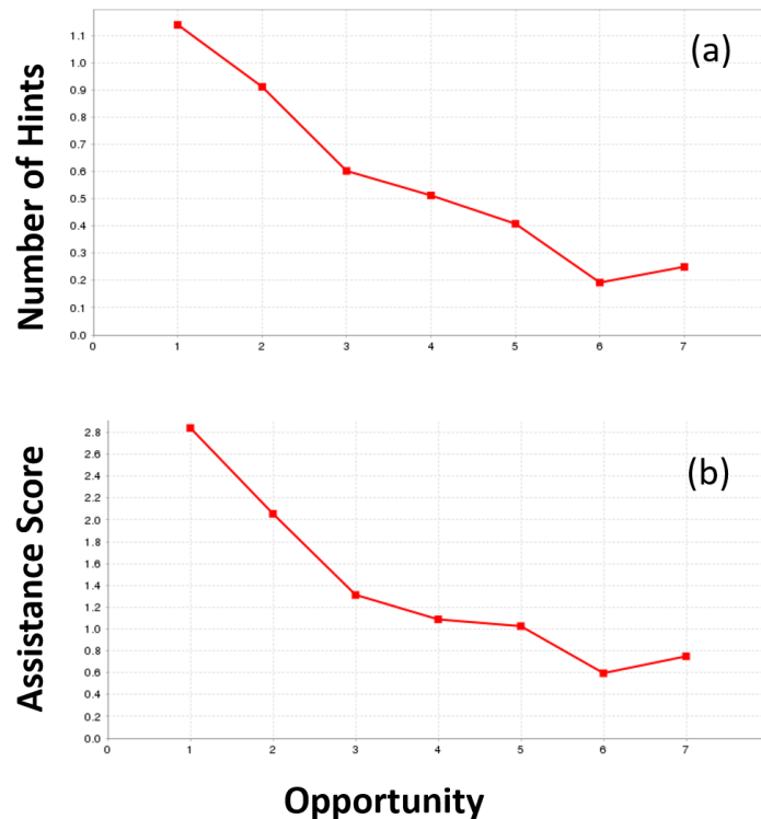
Figure 1. (a and b) Extent of assistance students need with successive opportunities and hints given by intelligent tutor
