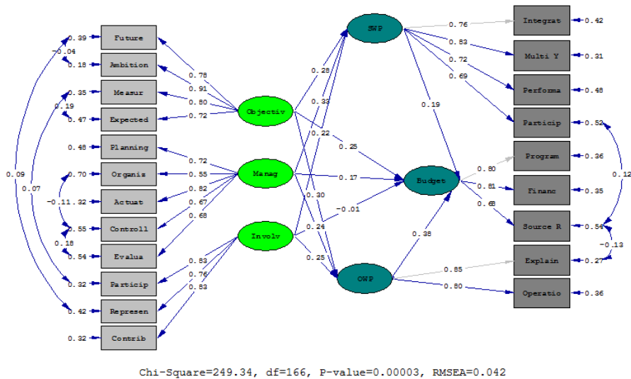
Figure 1 Structural Model of Standardized Solution
