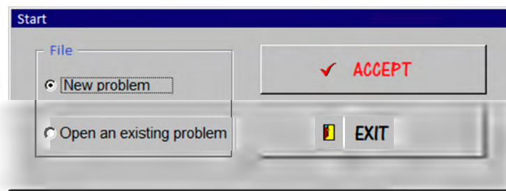
Figure 3. Start-up window.
