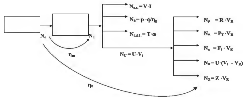
Figure 1. Power balance for a single-traction tractor.
