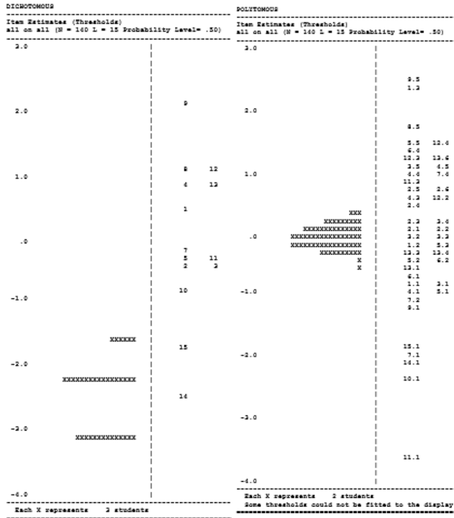
(a) (b) Figure 2. The mapping of the estimation of the upper secondary school students' ability and the item difficulty for (a) dichotomous scoring and (b) polytomous scoring
