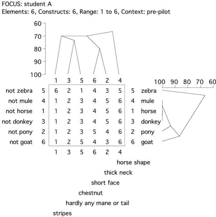
Figure 4. Output of FOCUS program of the RepGrid 2.0 package
