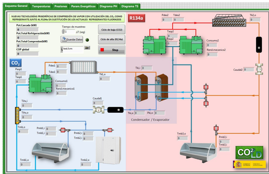
Figure 9. Front end of the DAQ system
