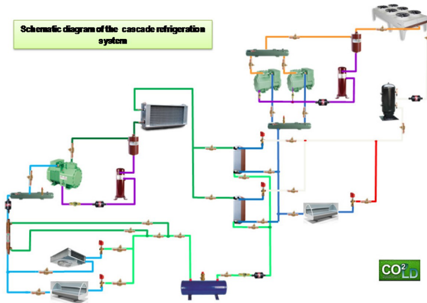
Figure 4. Schematic diagram of the design of the cascade refrigeration systems
