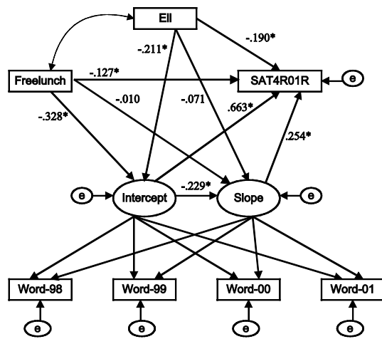
Figure 2. Conditional LGM with Parameter Estimates: Representing the Prediction of SAT-9 Scores in 4th Grade from Oral Reading Fluency Scores Across Grades 1 st - 4 th , Considering Free and Reduced Lunch among English Language Learner Students.
